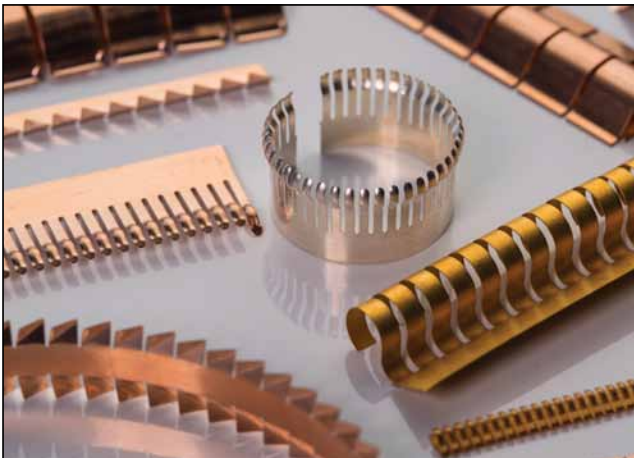
High-performance finger-stock gaskets from Orbel deliver the industry's highest EMI shielding effectiveness and are available in a variety of materials.
