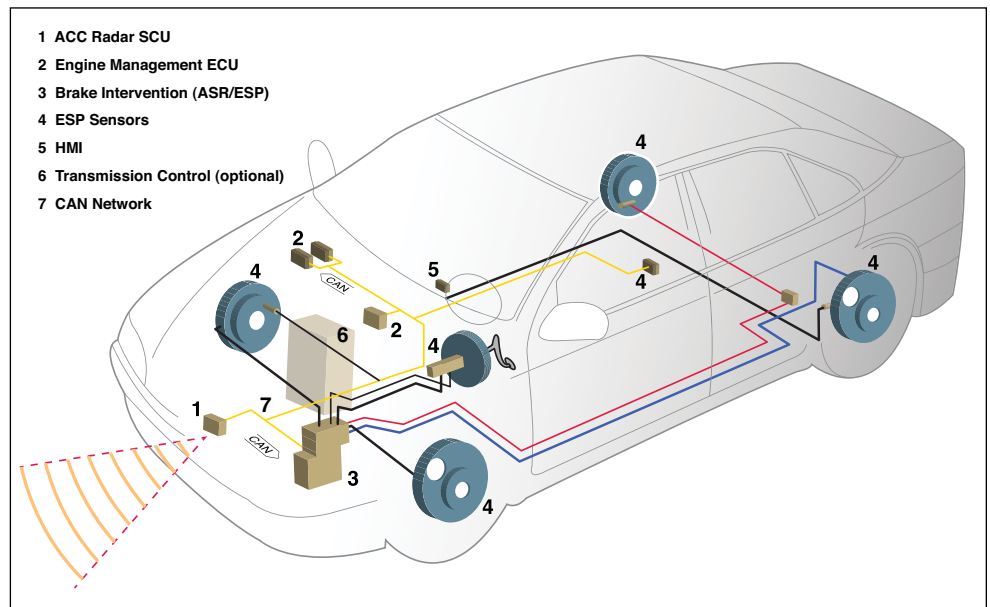
Overview of EMI-sensitive automotive systems.
